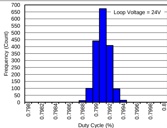
Figure 11. 0.8% Duty Cycle Distribution, NPN Mode
