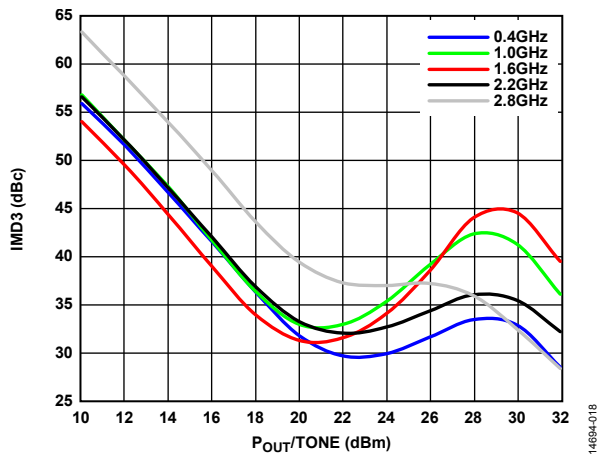
Figure 18. Output Third-Order Intermodulation (IMD3) vs. P_{OUT}/Tone at V_{DD} = 28\text{ V}
