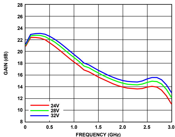
Figure 7. Gain vs. Frequency at Various Supply Voltages
