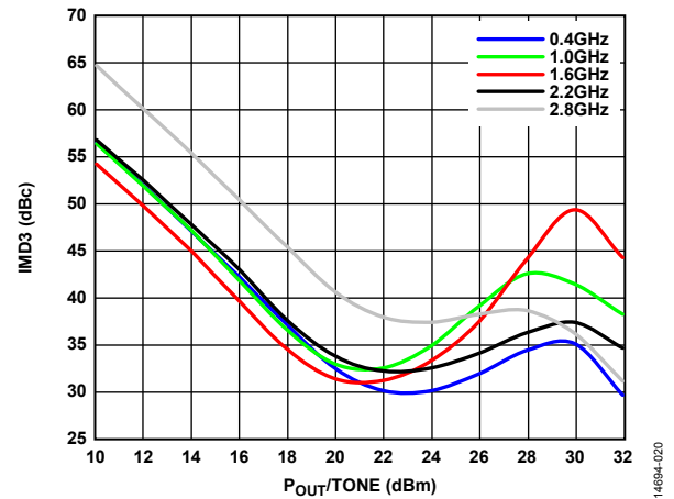
Figure 20. Output Third-Order Intermodulation (IMD3) vs. P_{OUT}/Tone at V_{DD} = 32\text{ V}
