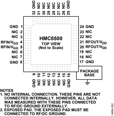
Figure 2. Pin Configuration
