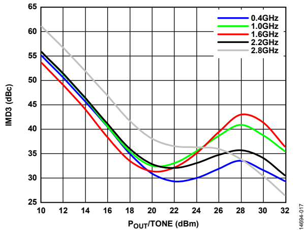
Figure 17. Output Third-Order Intermodulation (IMD3) vs. P_{OUT}/Tone at V_{DD} = 24\text{ V}
