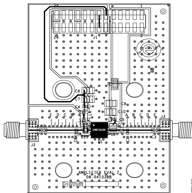
Figure 42. Evaluation PCB
