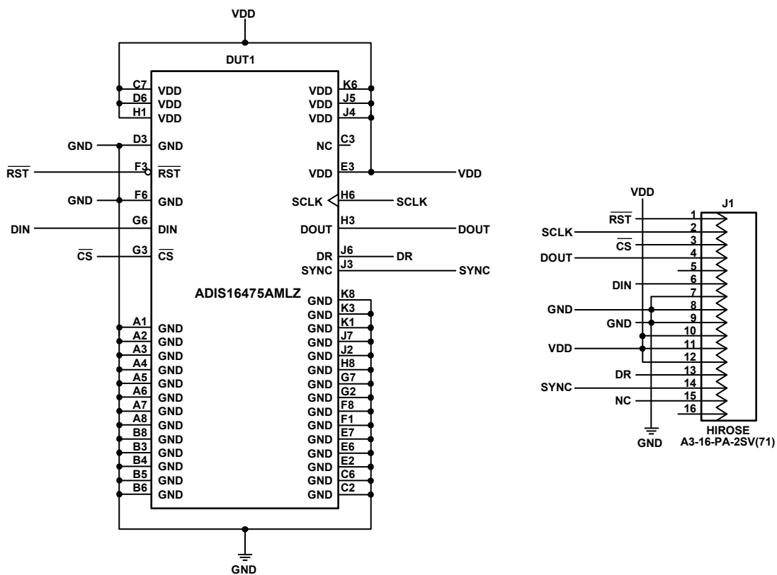
Figure 47. Breakout Board Schematic
