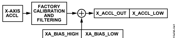
Figure 39. User Calibration Signal Path, Accelerometers
