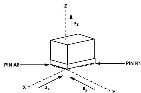
Figure 32. Accelerometer Axis and Polarity Assignments
