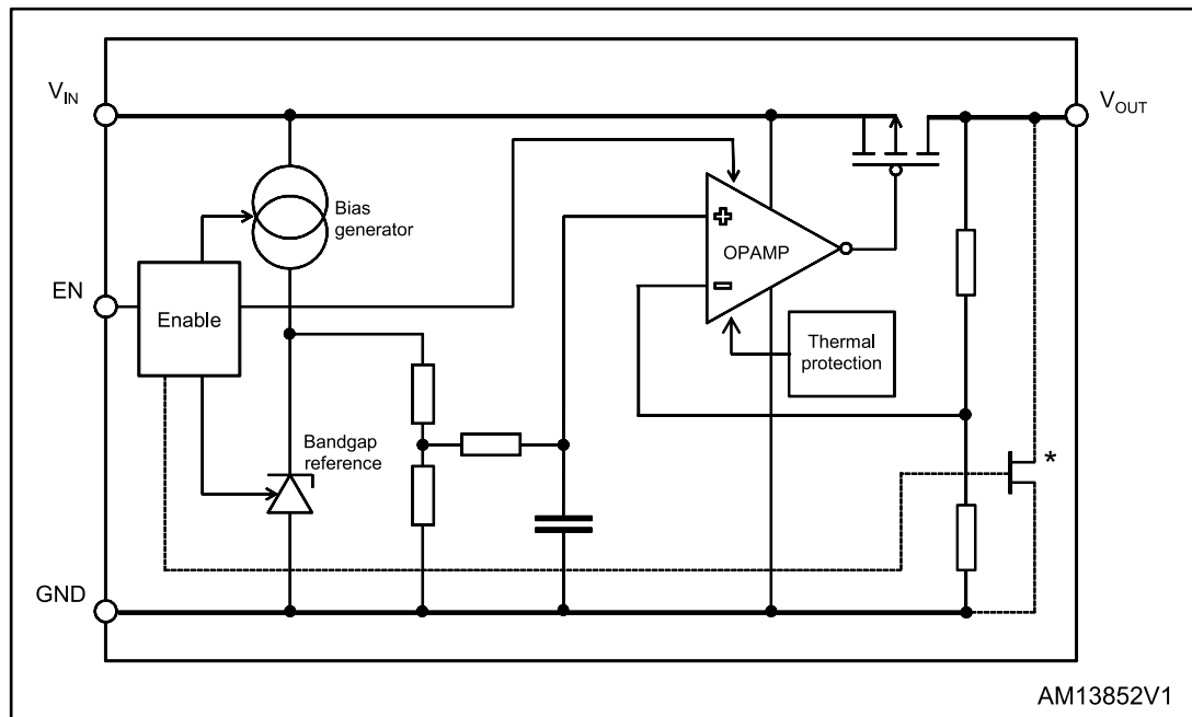
Figure 1: Block diagram
