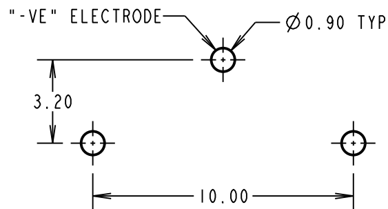
RECOMMENDED PCB LAYOUT (TOLERANCE \pm 0.05 )
